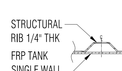
RIB LAMINATE DETAIL F NTS
