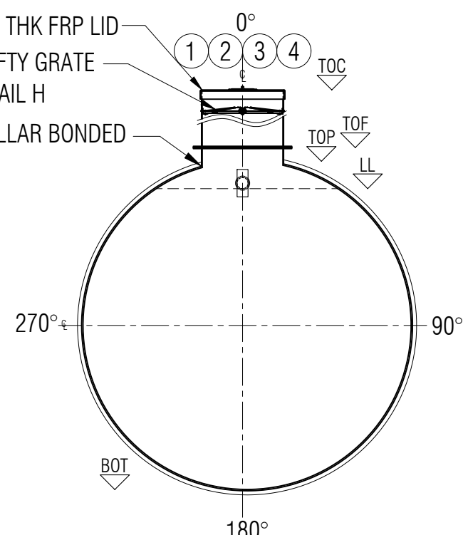
SECTION C
