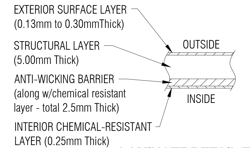
LAMINATE DETAIL E NTS
