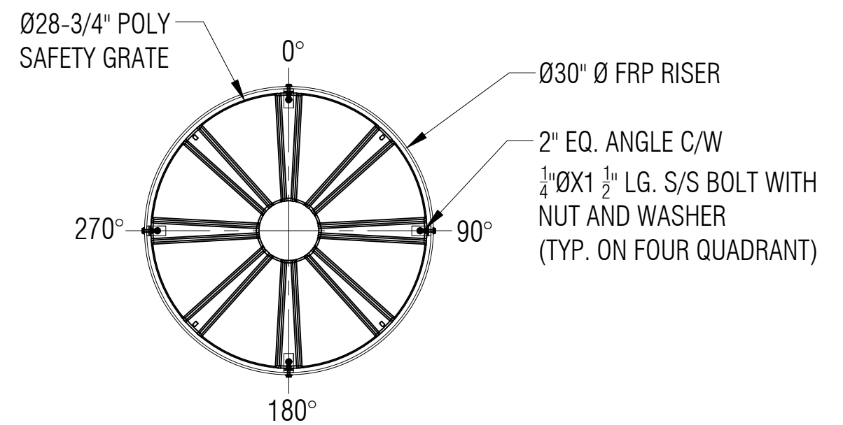
SAFETY GRATE DETAIL G SCALE: 1:15
