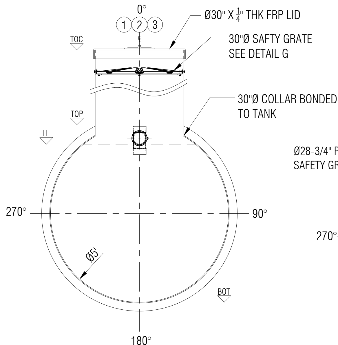
SECTION C
