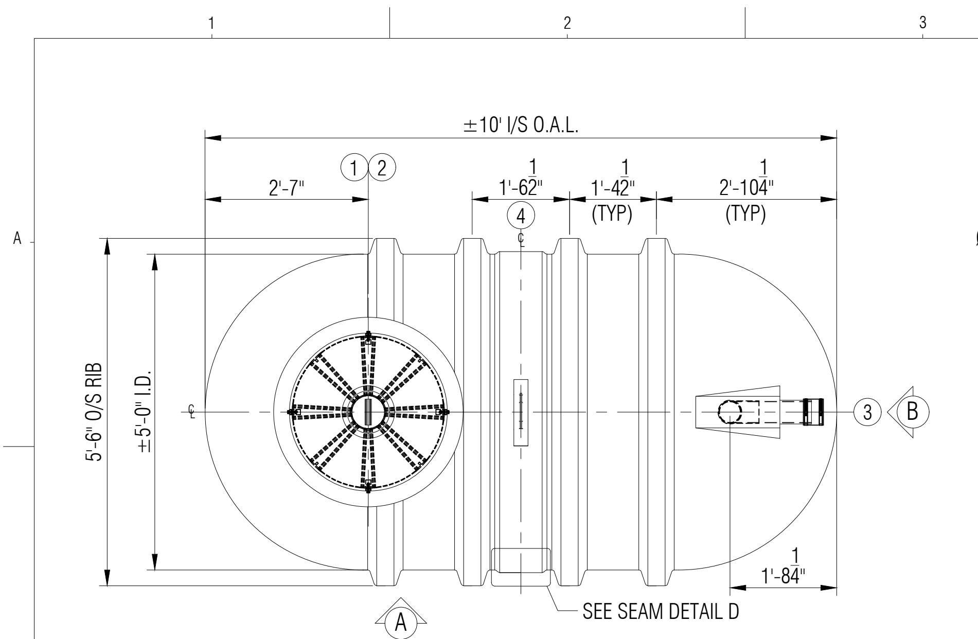
PLAN
