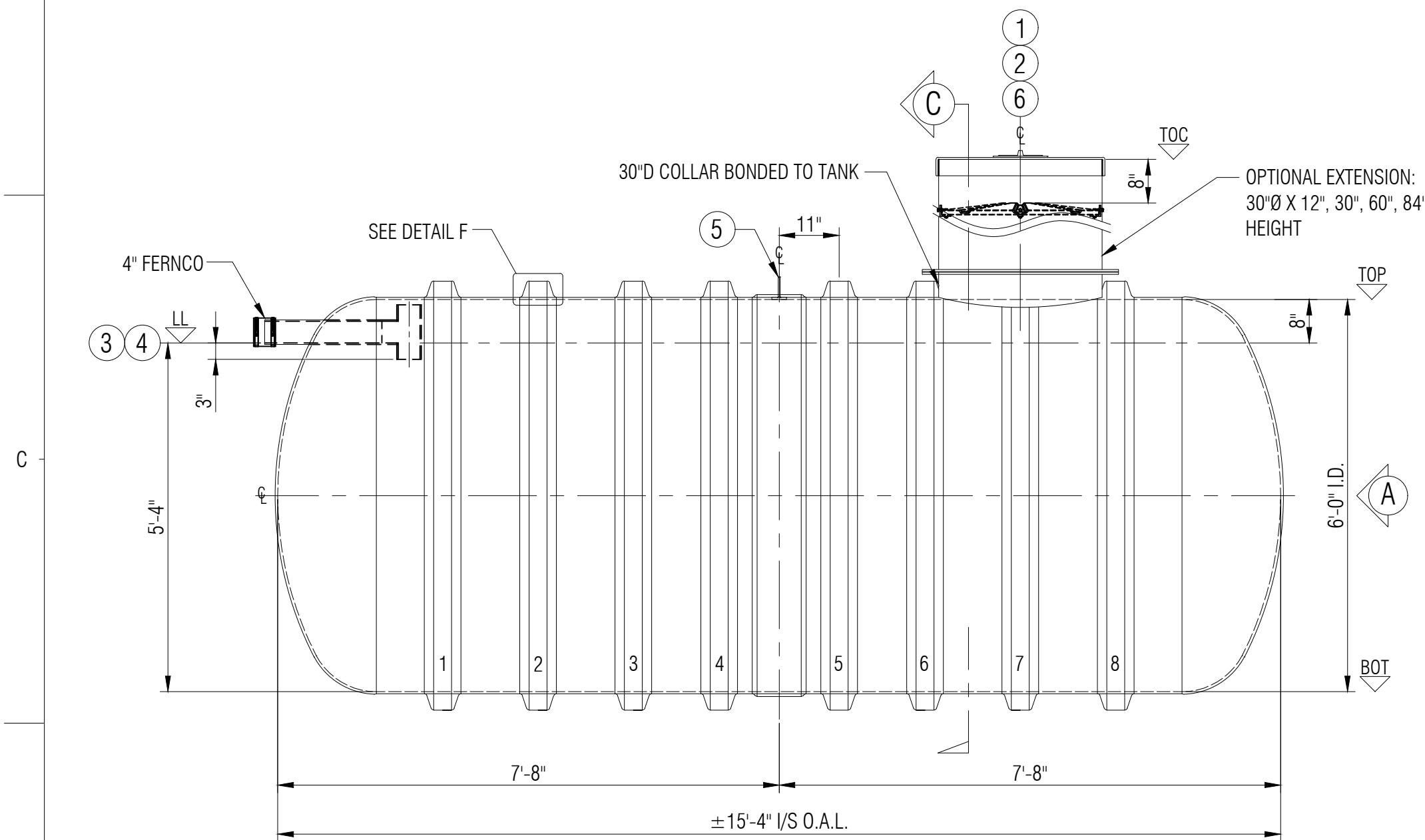
ELEVATION "A"
