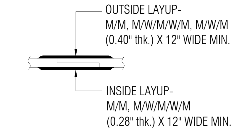
TYPICAL BODY JOINT DETAIL D NTS
