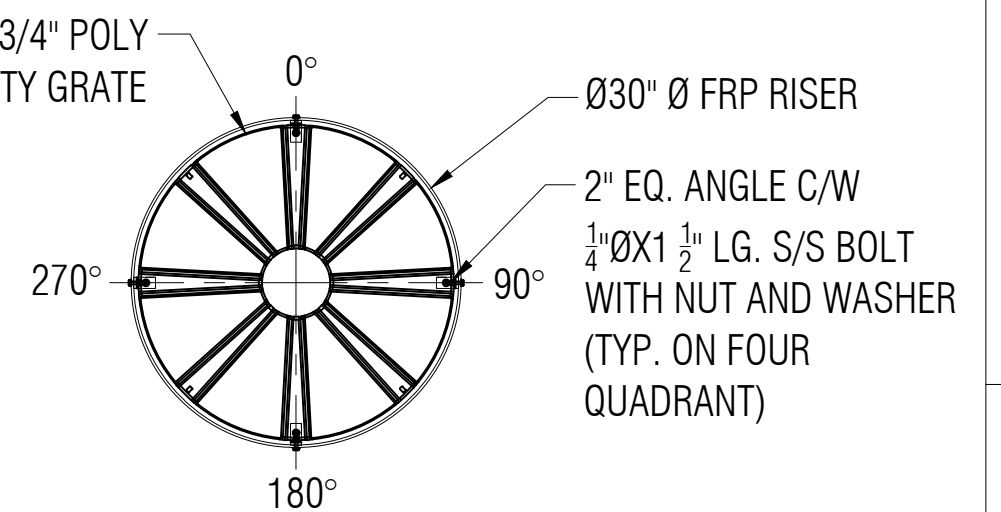
⑥ SAFETY GRATE DETAIL G SCALE: 1:15
