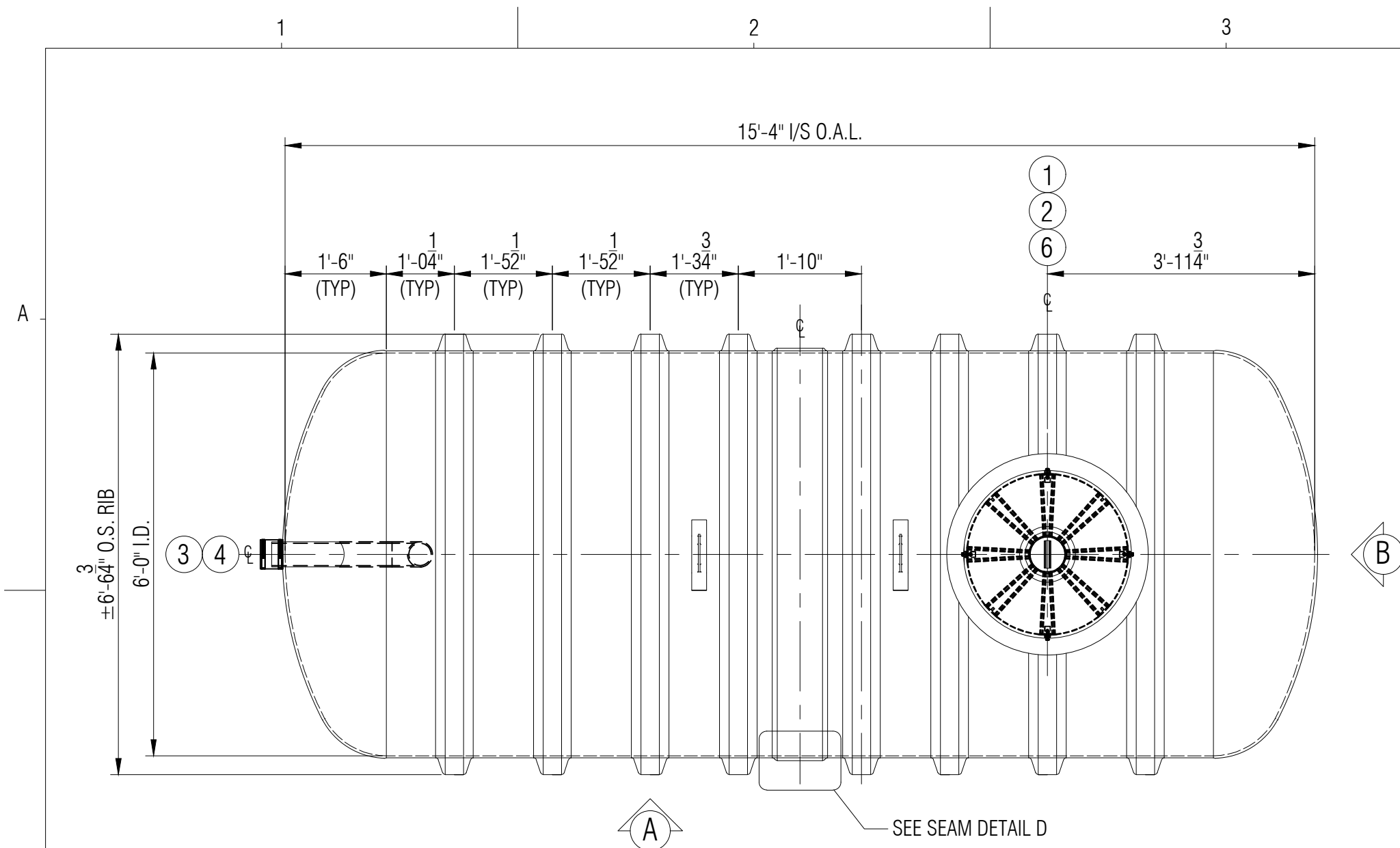
PLAN
