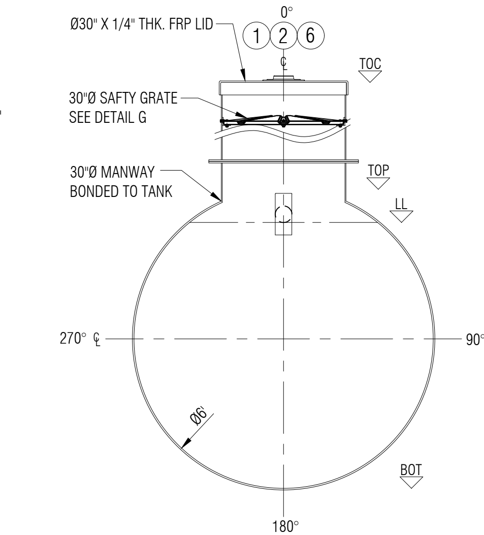
SECTION "C"
