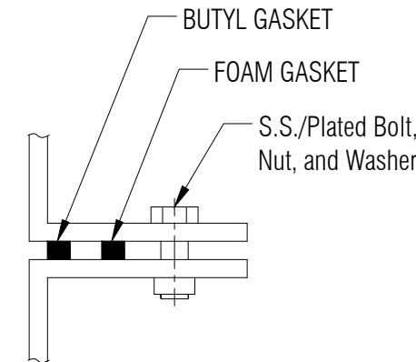
FLANGE TO FLANGE CONNECTION DETAIL 2 NTS
