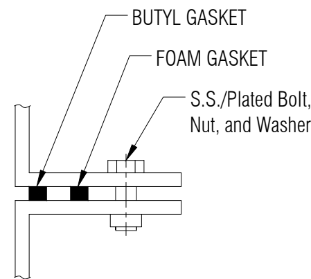
FLANGE TO FLANGE CONNECTION DETAIL 2 N T S
