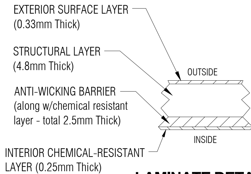
LAMINATE DETAIL 1 N T S
