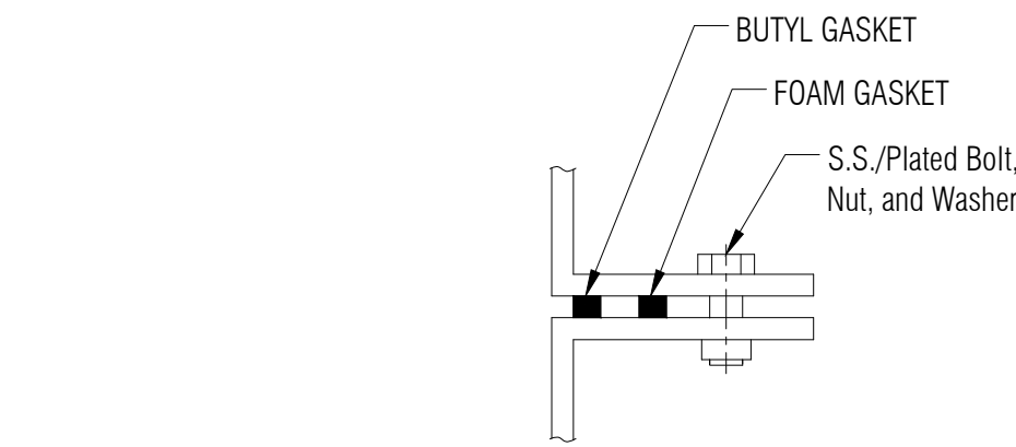
FLANGE TO FLANGE CONNECTION DETAIL 2 NTS
