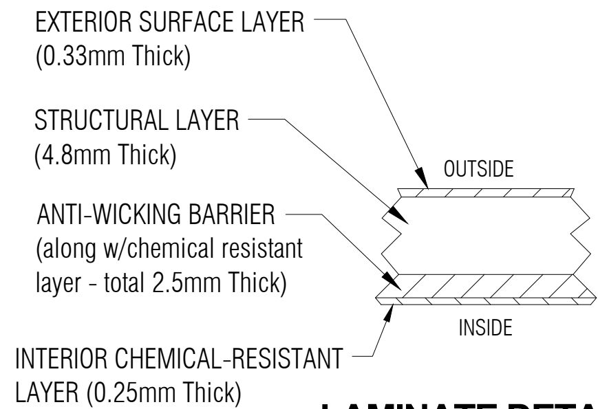
LAMINATE DETAIL 1 NTS
