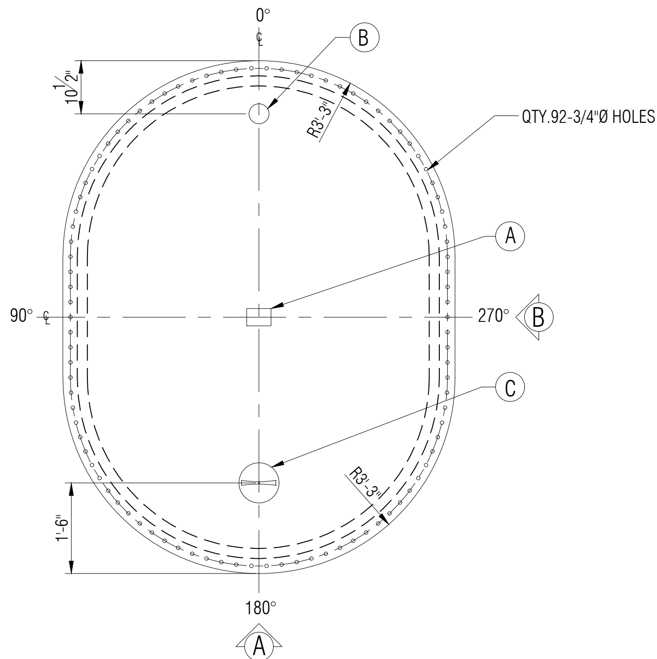
PLAN
