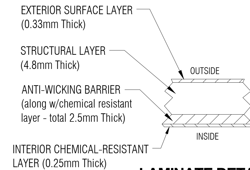
LAMINATE DETAIL 1
