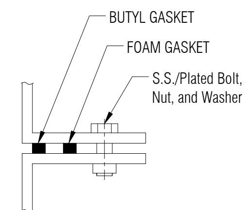
FLANGE TO FLANGE CONNECTION DETAIL 2
