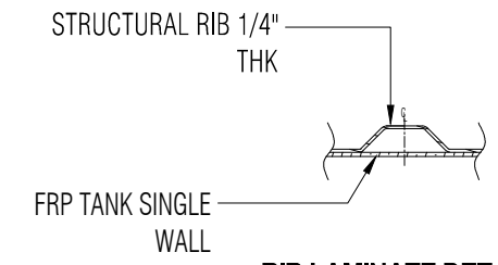
RIB LAMINATE DETAIL F NTS
