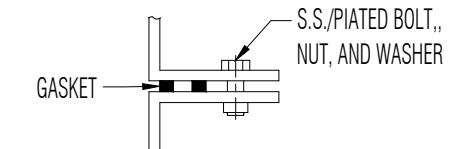
FLANGE TO FLANGE CONNECTION DETAIL G NTS
