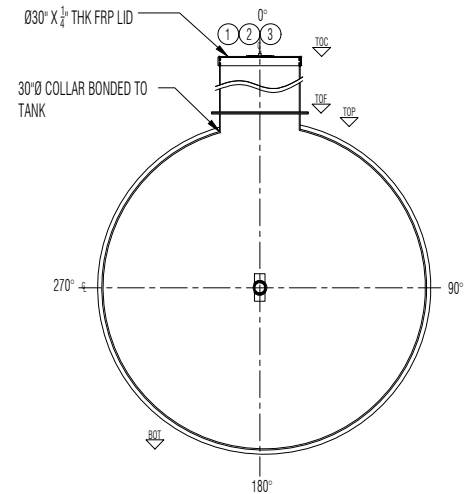
SECTION C
