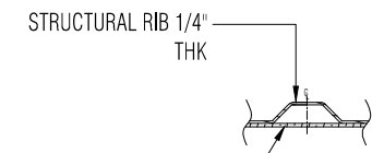
RIB LAMINATE DETAIL F NTS
