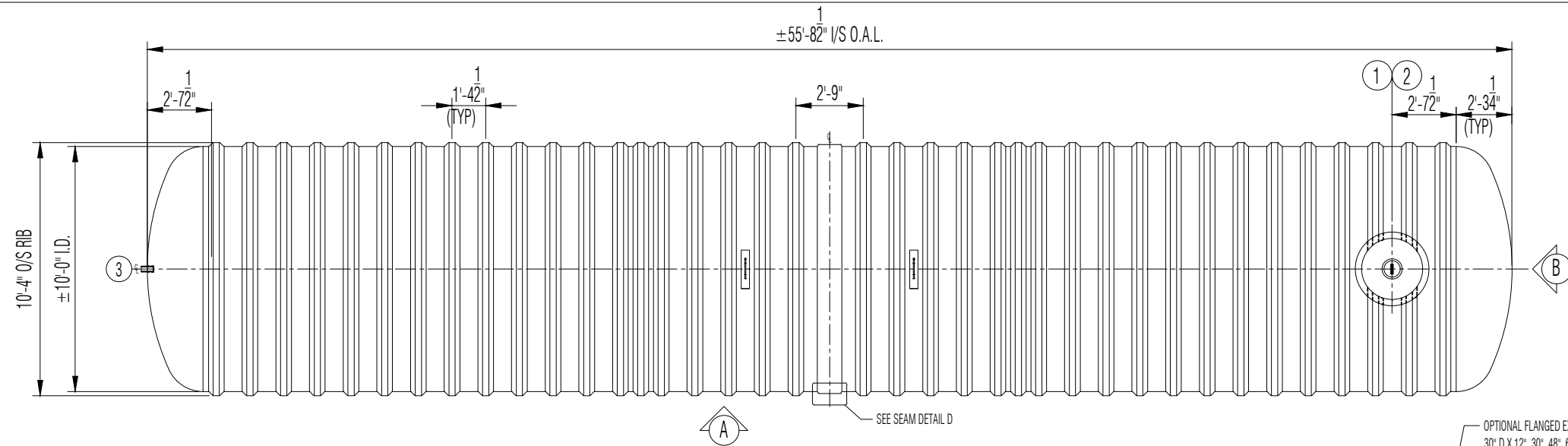
PLAN
