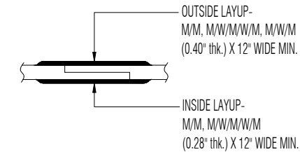
TYPICAL BODY JOINT DETAIL D NTS
