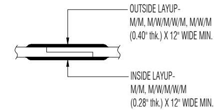
TYPICAL BODY JOINT DETAIL D
