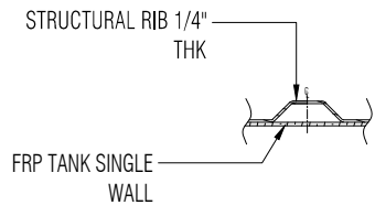
RIB LAMINATE DETAIL F
