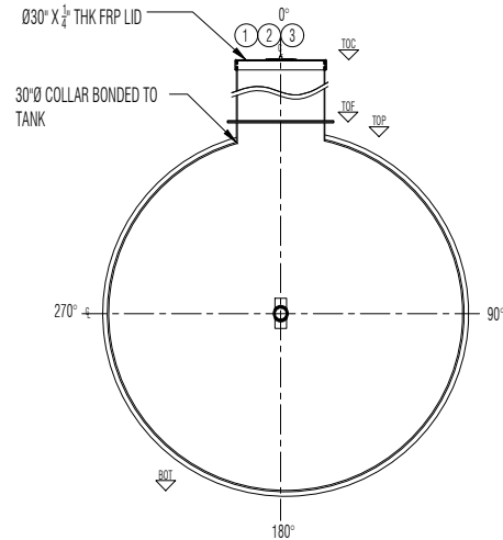
SECTION C
