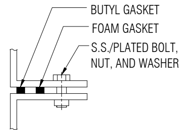
FLANGE TO FLANGE CONNECTION DETAIL 2 NTS
