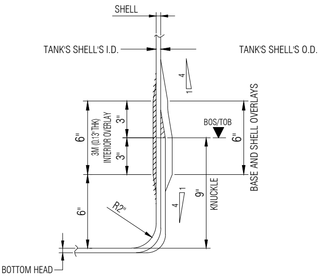
KNUCKLE/BASE/TOP/SHELL DETAIL 3 NTS
