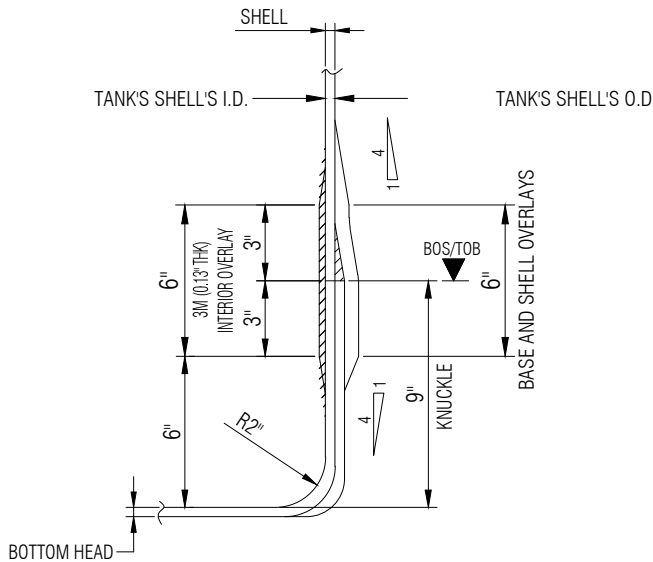
KNUCKLE/BASE/TOP/SHELL DETAIL 3 NTS
