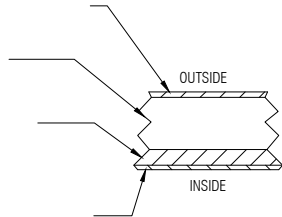
LAMINATE DETAIL 1 NTS
