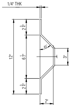
SHELL RIB DETAIL 4 NTS
