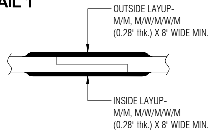
TYPICAL BODY JOINT DETAIL 2
