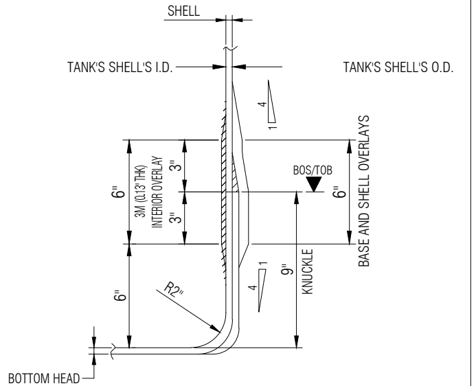
KNUCKLE/BASE/TOP/SHELL DETAIL 3 NTS
