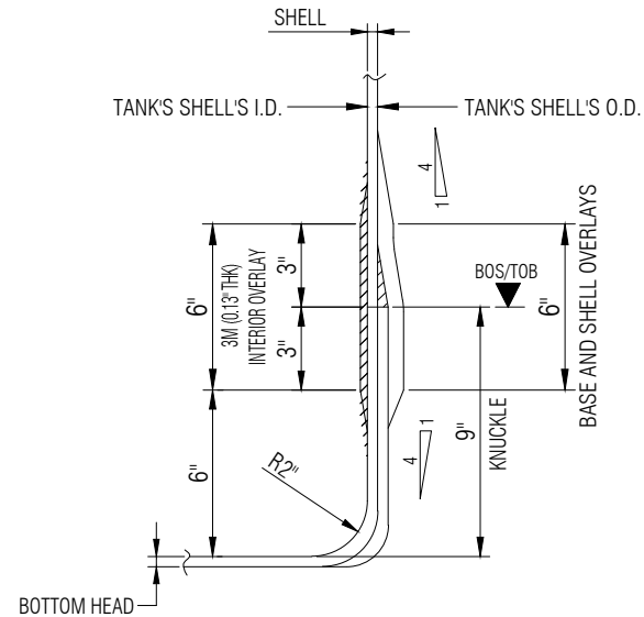
KNUCKLE/BASE/TOP/SHELL DETAIL 3 NTS
