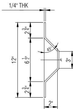
SHELL RIB DETAIL 4 NTS
