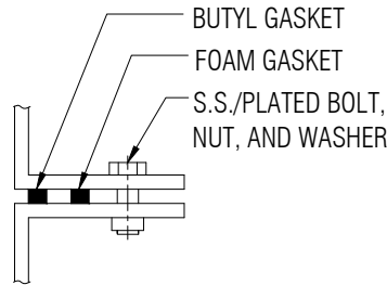
FLANGE TO FLANGE CONNECTION DETAIL 2 NTS
