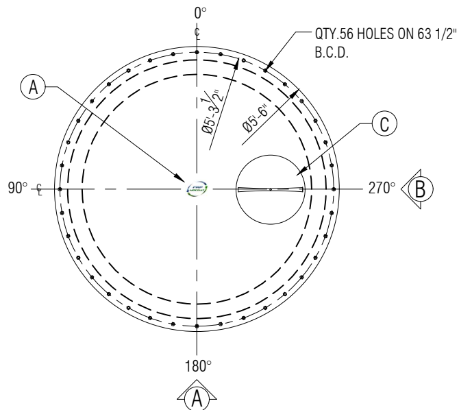
PLAN
