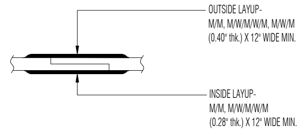
TYPICAL BODY JOINT DETAIL DETAIL D S105 NTS
