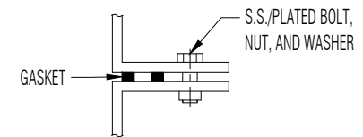
FLANGE TO FLANGE CONNECTION DETAIL F S107 NTS
