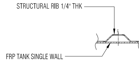
RIB LAMINATE DETAIL DETAIL G S108 NTS
