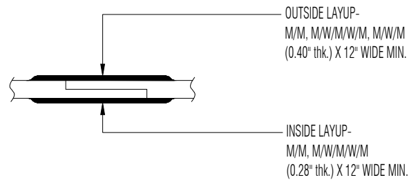
TYPICAL BODY JOINT DETAIL DETAIL D NTS
