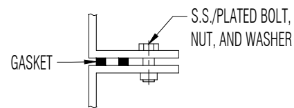
FLANGE TO FLANGE CONNECTION DETAIL F NTS
