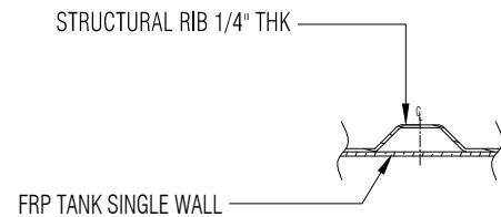
RIB LAMINATE DETAIL DETAIL G NTS
