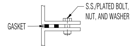
FLANGE TO FLANGE CONNECTION DETAIL F NTS
