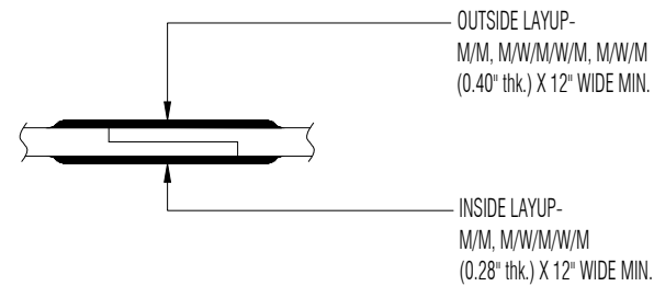
TYPICAL BODY JOINT DETAIL DETAIL D
