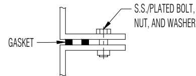
FLANGE TO FLANGE CONNECTION DETAIL F
