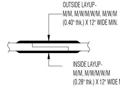
TYPICAL BODY JOINT DETAIL DETAIL D
