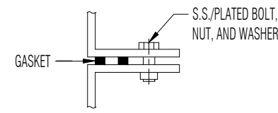
FLANGE TO FLANGE CONNECTION DETAIL F
