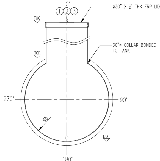
SECTION C
