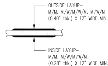
TYPICAL BODY JOINT DETAIL D
