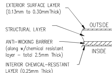
LAMINATE DETAIL E
