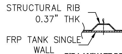
RIB LAMINATE DETAIL F N T S
