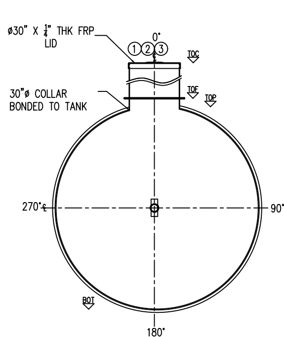
SECTION C
