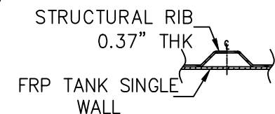
RIB LAMINATE DETAIL F N T S
