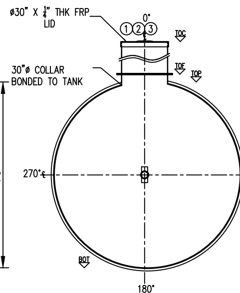
SECTION C
