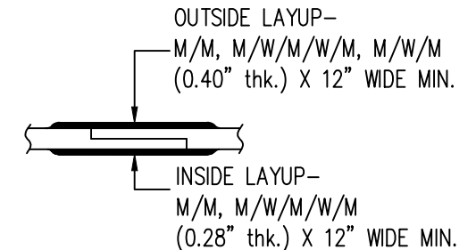
TYPICAL BODY JOINT DETAIL D N T S
