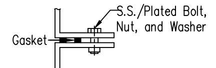
FLANGE TO FLANGE CONNECTION DETAIL G N T S
