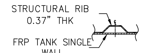
RIB LAMINATE DETAIL F N T S
