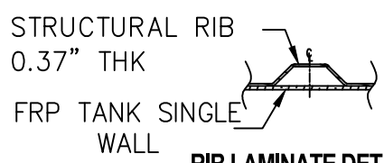
RIB LAMINATE DETAIL F N T S
