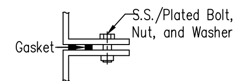
FLANGE TO FLANGE CONNECTION DETAIL G N T S
