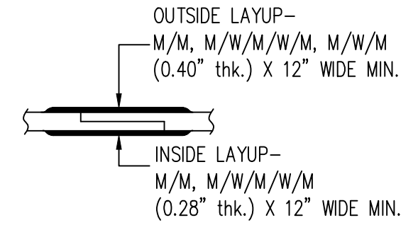
TYPICAL BODY JOINT DETAIL D N T S
