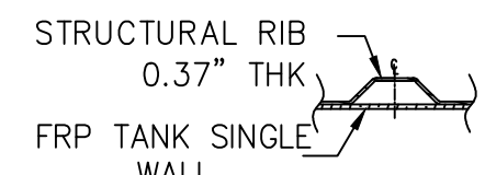
RIB LAMINATE DETAIL F N T S
