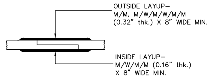
BODY JOINT DETAIL C
