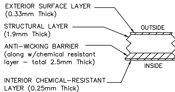
LAMINATE DETAIL D N T S
