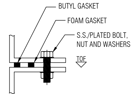
FLANGE TO FLANGE CONNECTION DETAIL 2 NTS
