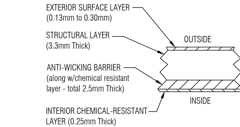
LAMINATE DETAIL 1 NTS
