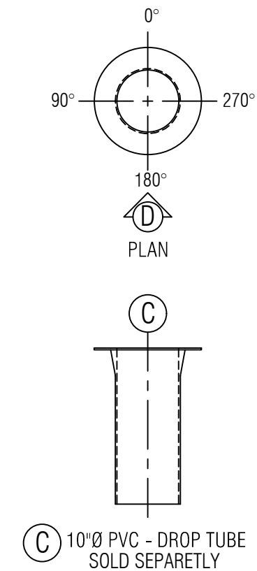
ELEVATION D
