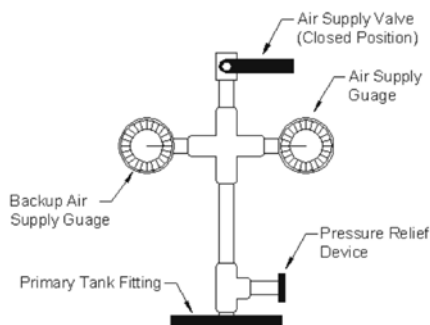
Tank Test Manifold
