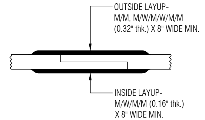
BODY JOINT DETAIL 1
