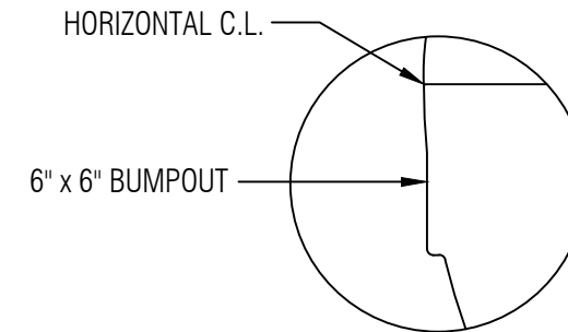
DETAIL 3
