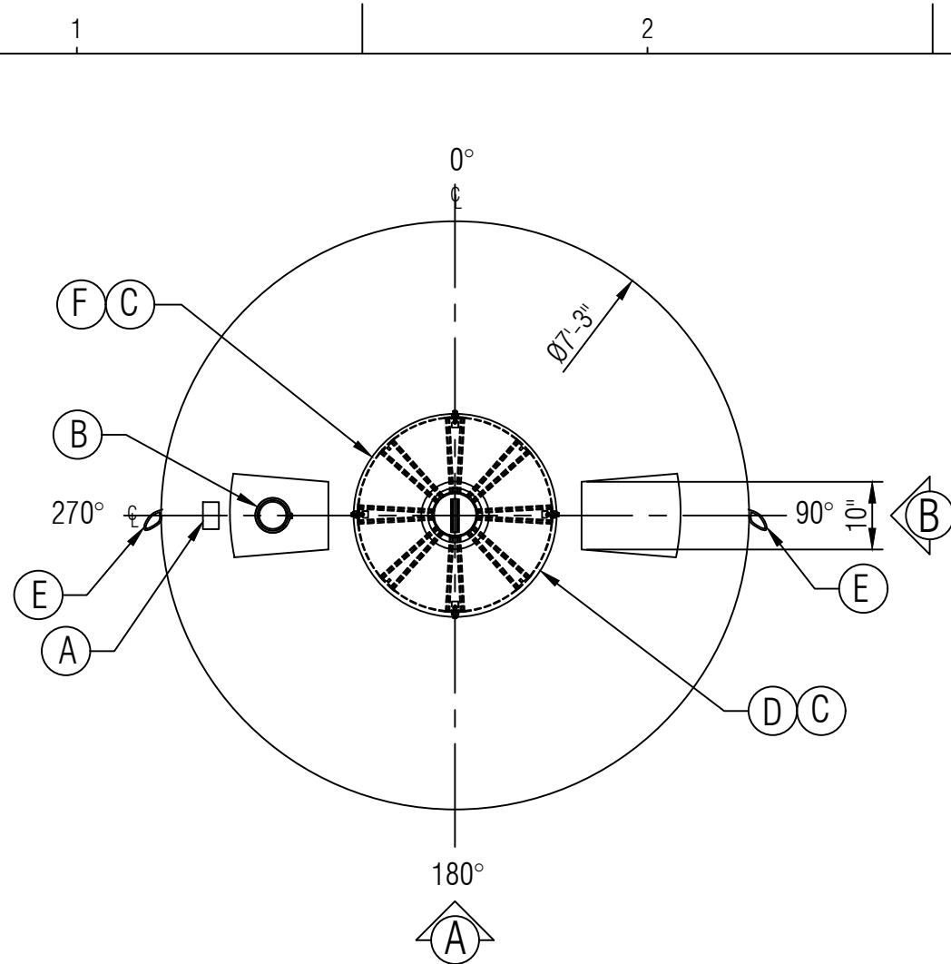
PLAN
