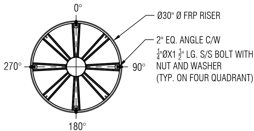
SAFETY GRATE DETAIL 2
