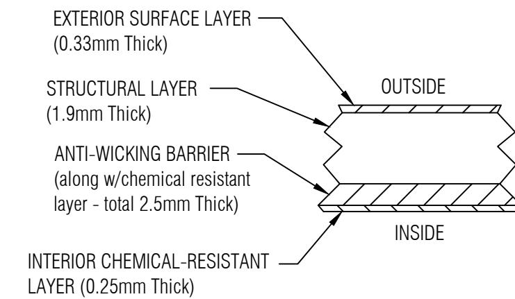
LAMINATE DETAIL 4 NTS
