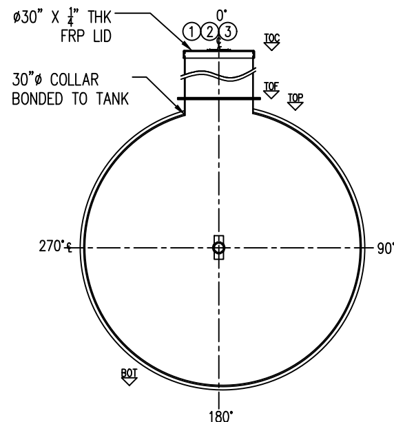
SECTION C
