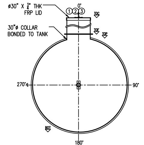
SECTION C
