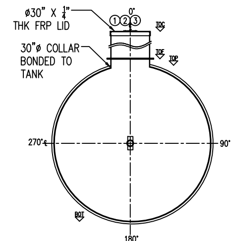
SECTION C
