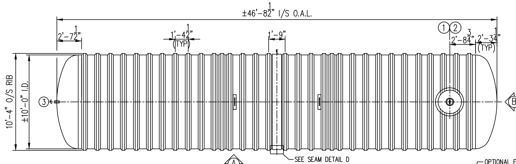
PLAN
