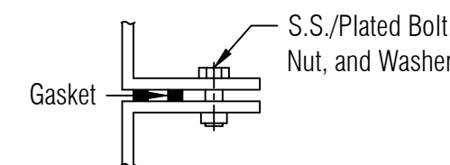
FLANGE TO FLANGE CONNECTION DETAIL G
