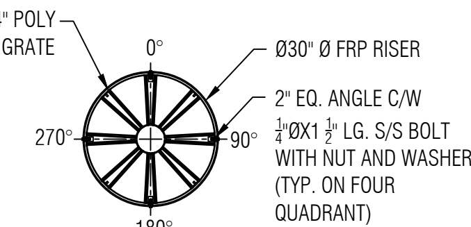
SAFETY GRATE DETAIL H
