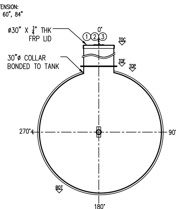
SECTION C
