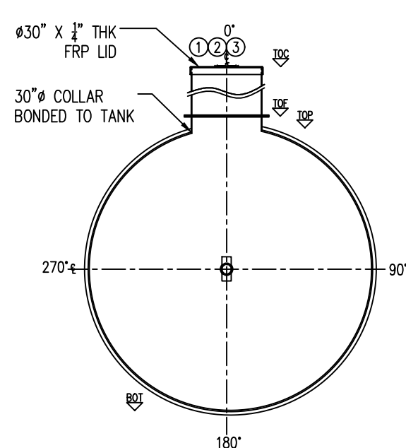
SECTION C
