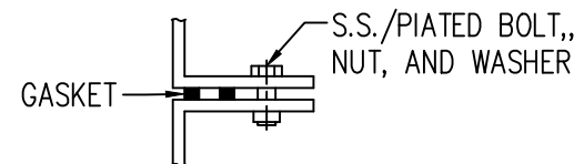
FLANGETO FLANGE CONNECTION DETAIL G N T S
