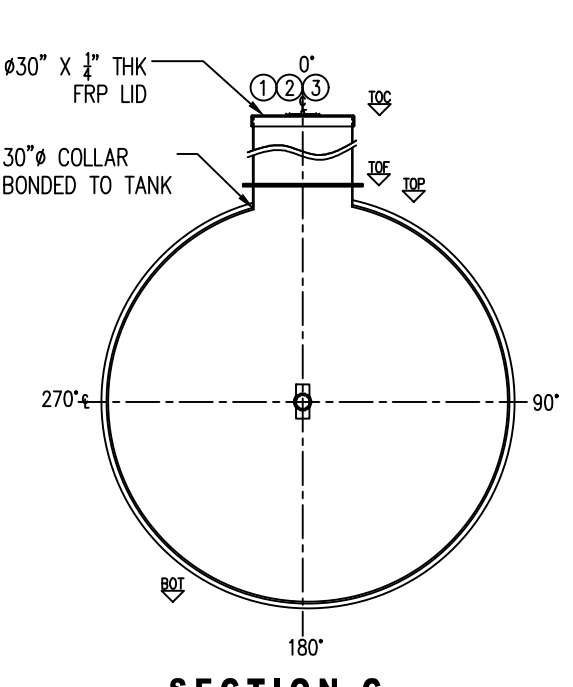
SECTION C
