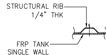
SECTION B
