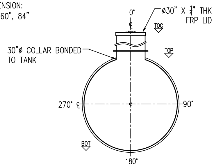
SECTION B
