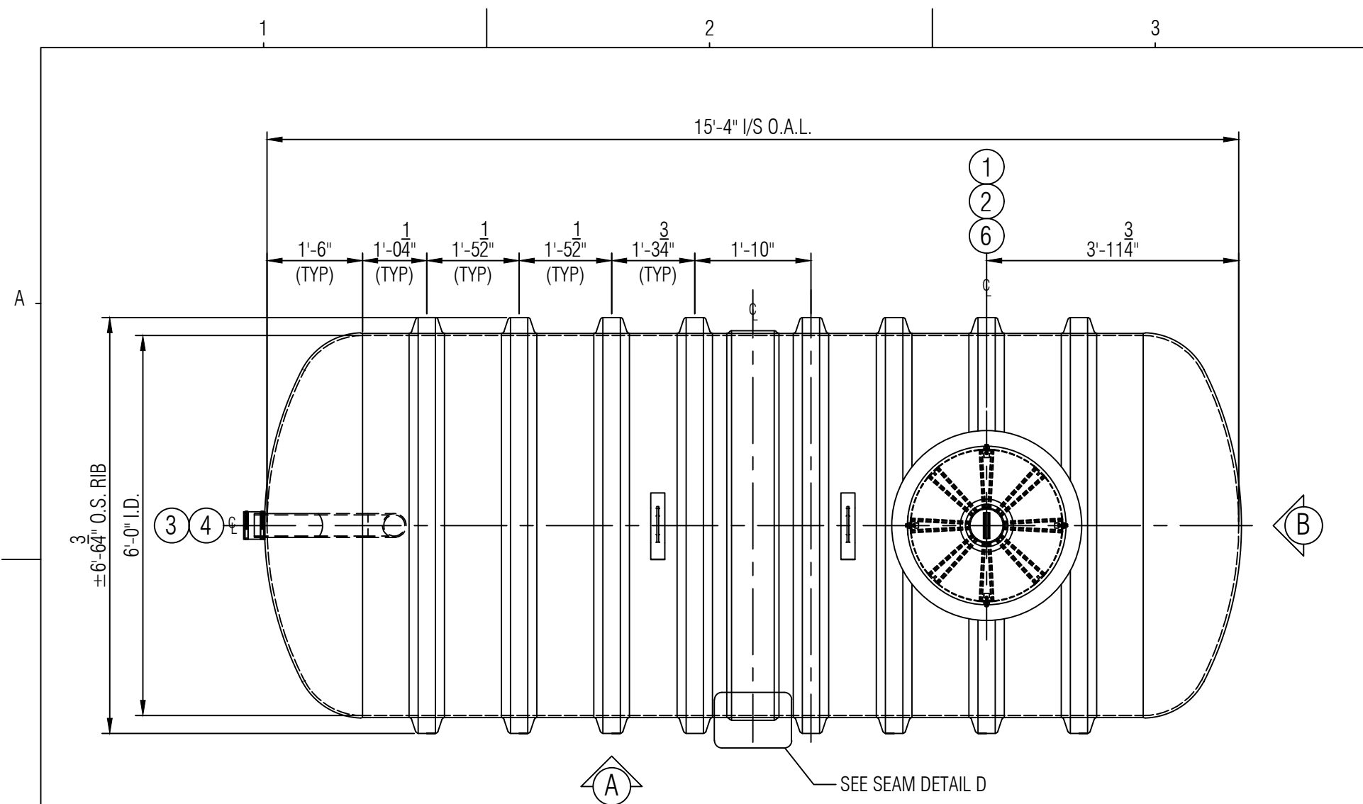
PLAN
