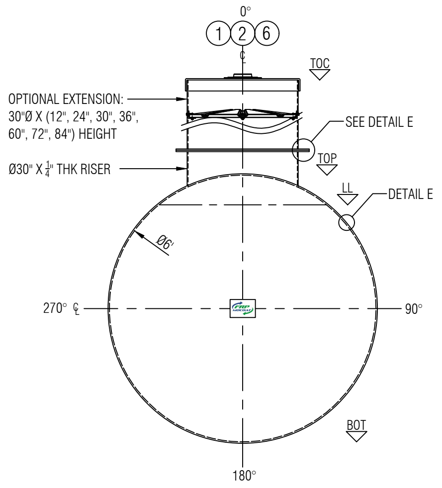
ELEVATION "B"
