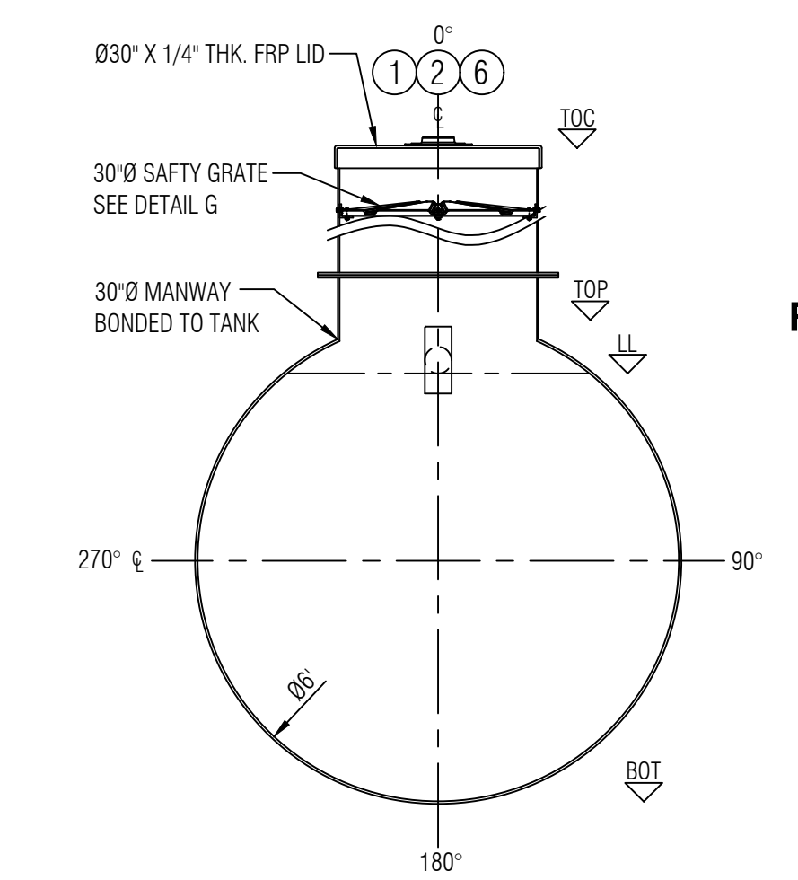
SECTION "C"
