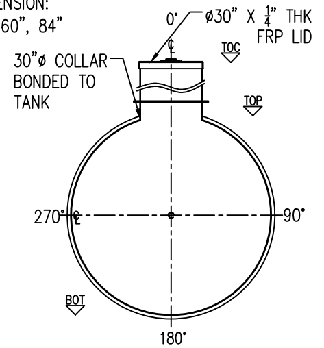
SECTION B
