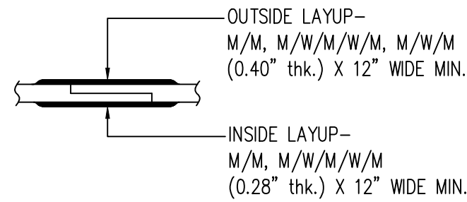
TYPICAL BODY JOINT DETAIL C N T S
