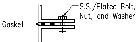
FLANGE TO FLANGE CONNECTION DETAIL E N T S
