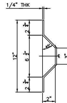
SHELL RIB DETAIL 4 N T S
