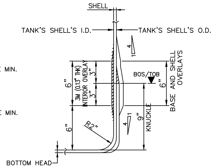
KNUCKLE/BASE/TOP/SHELL DETAIL 3 N T S
