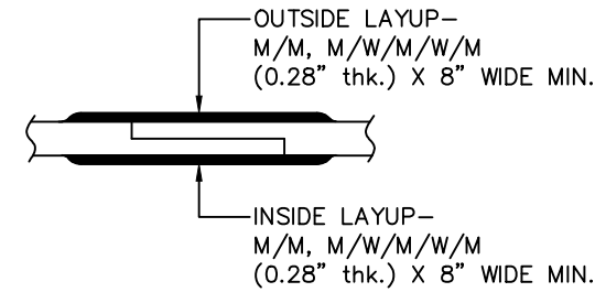
TYPICAL BODY JOINT DETAIL 2
