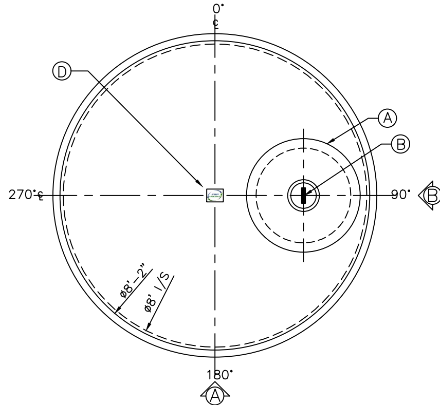
PLAN
