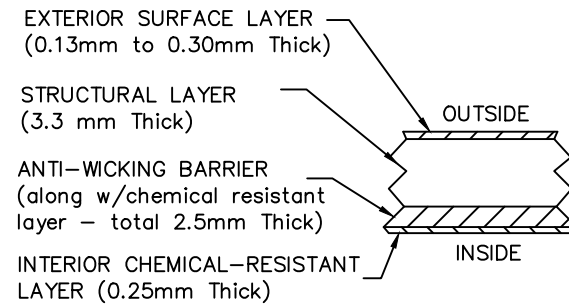
LAMINATE DETAIL 1 N T S
