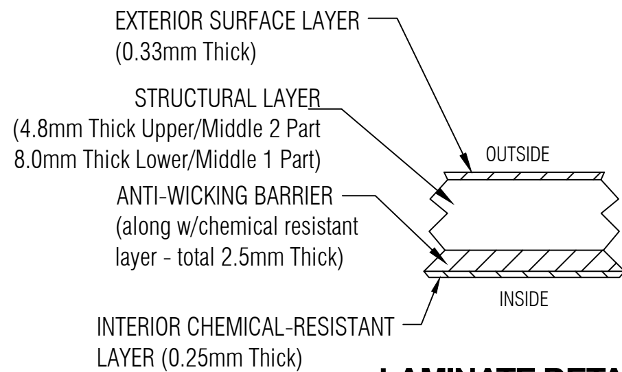
LAMINATE DETAIL 1 NTS
