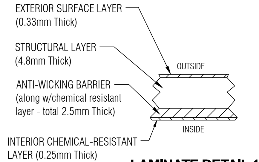
LAMINATE DETAIL 1 NTS
