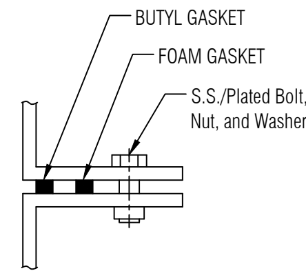
FLANGE TO FLANGE CONNECTION DETAIL 2 NTS
